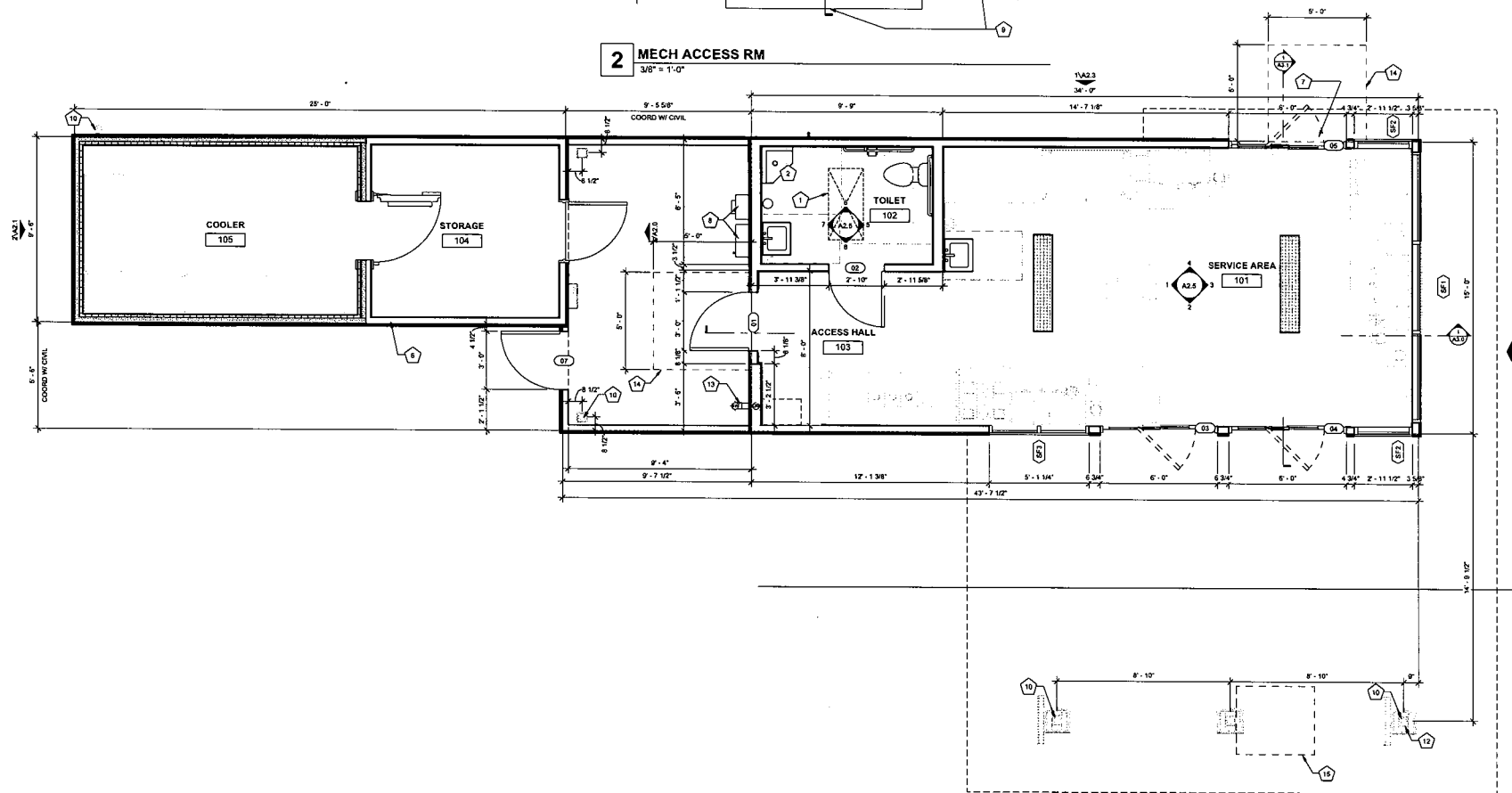
1 FLOOR PLAN 3/8" = 1'-0"
